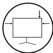
4-Sided Border
